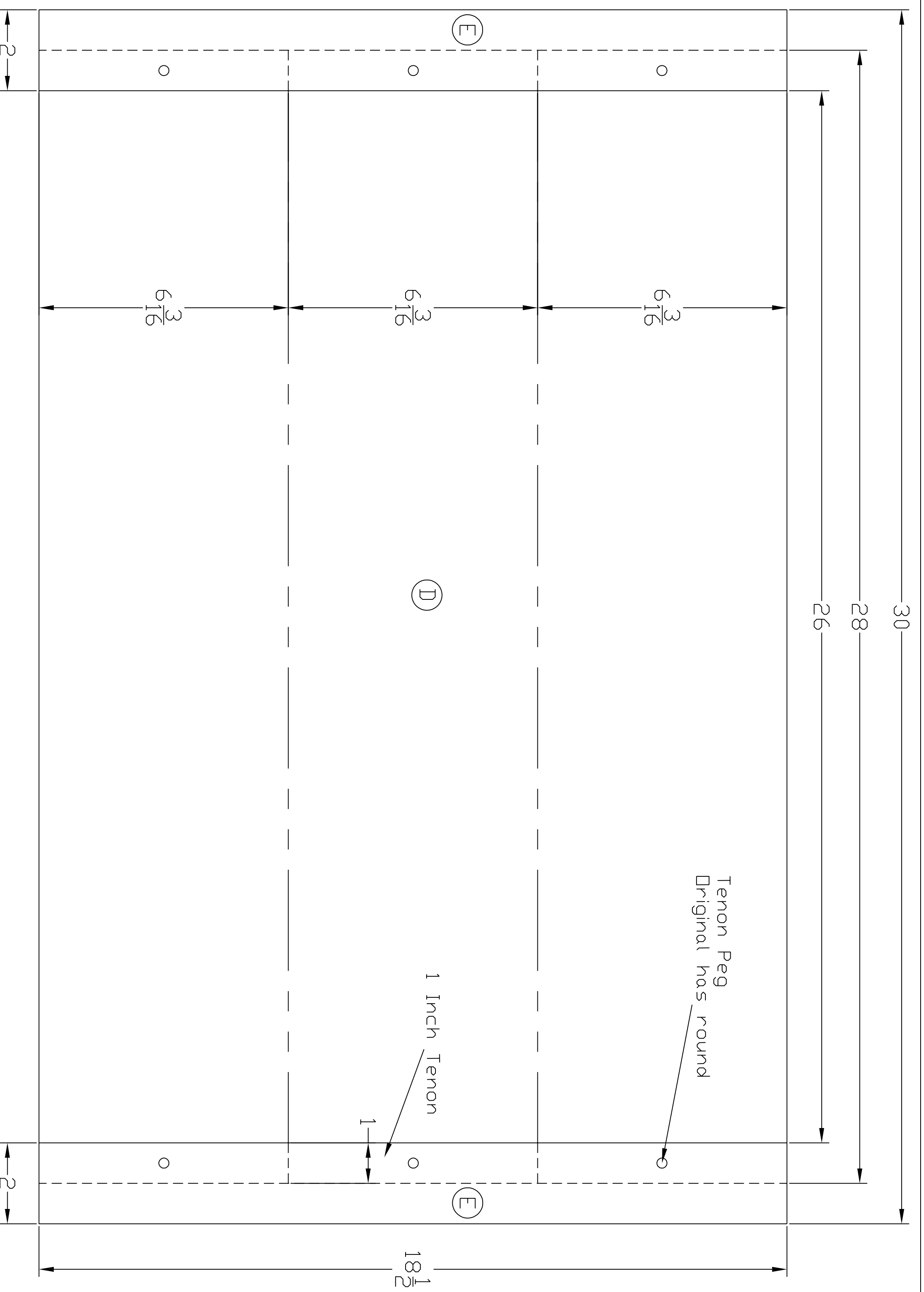
Stump Creek Mule Chest Top with dimensions
