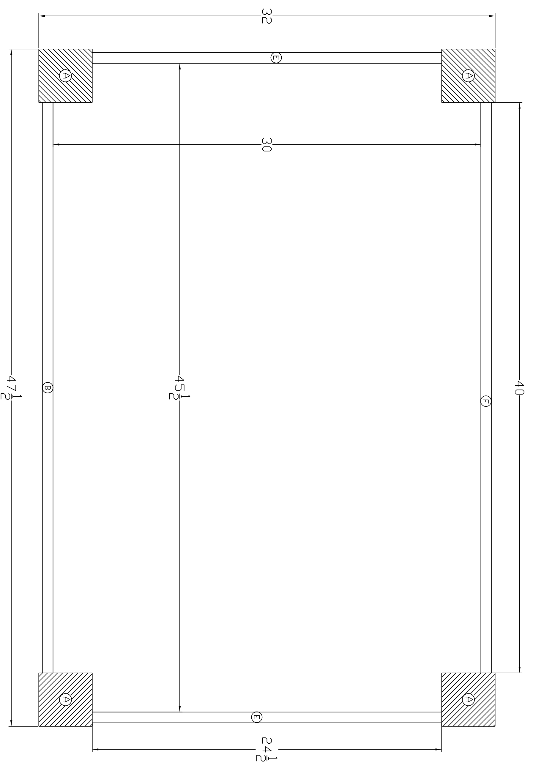
View: work station inner dimensions
