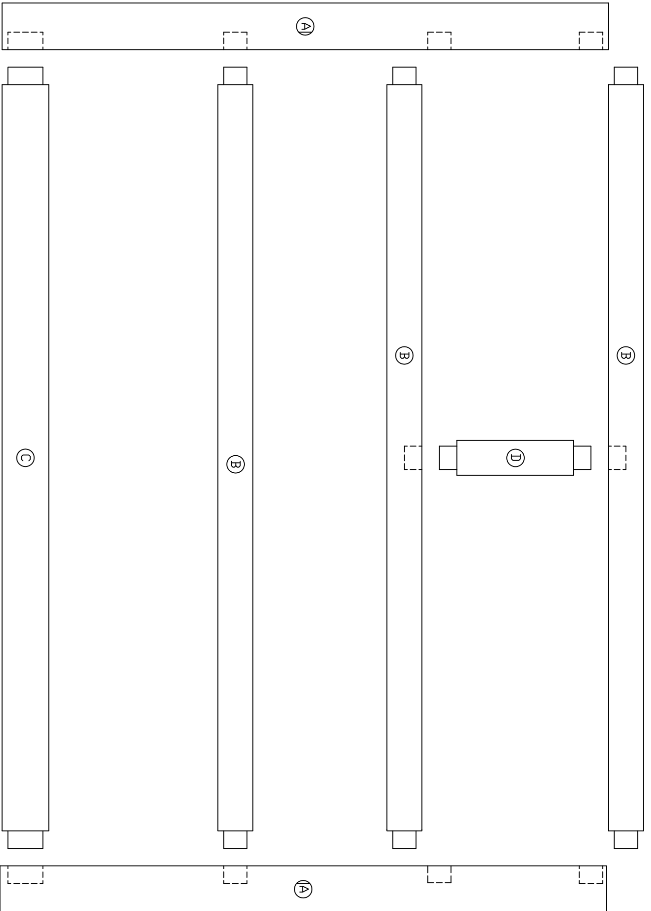
View: shaker chest of drawers open face frames
