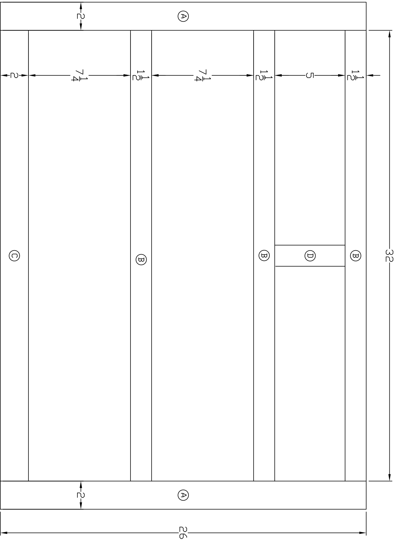
View: shaker chest of drawers face frames with dimensions
