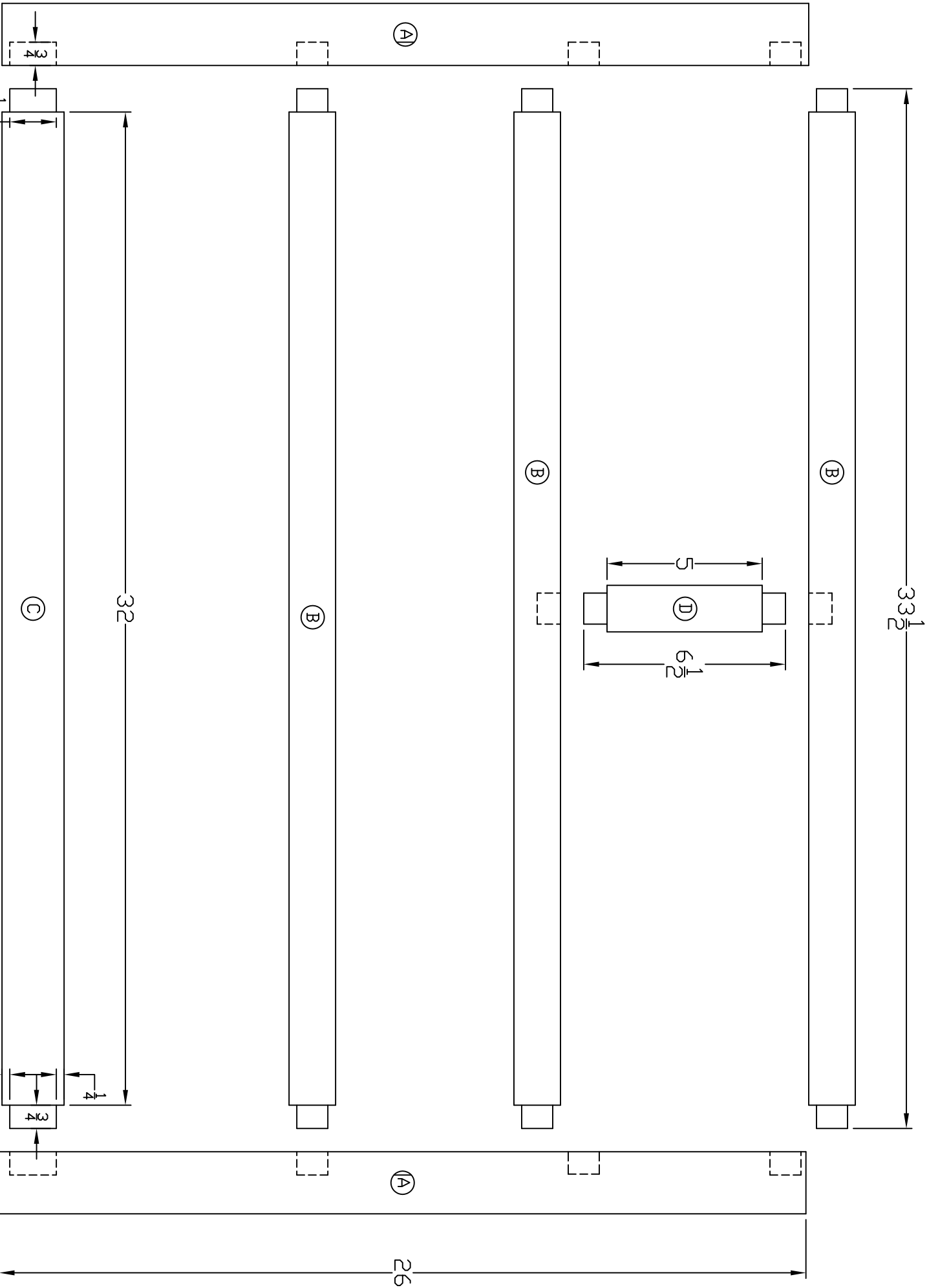
View: shaker chest of drawers open face frames with dimensions
