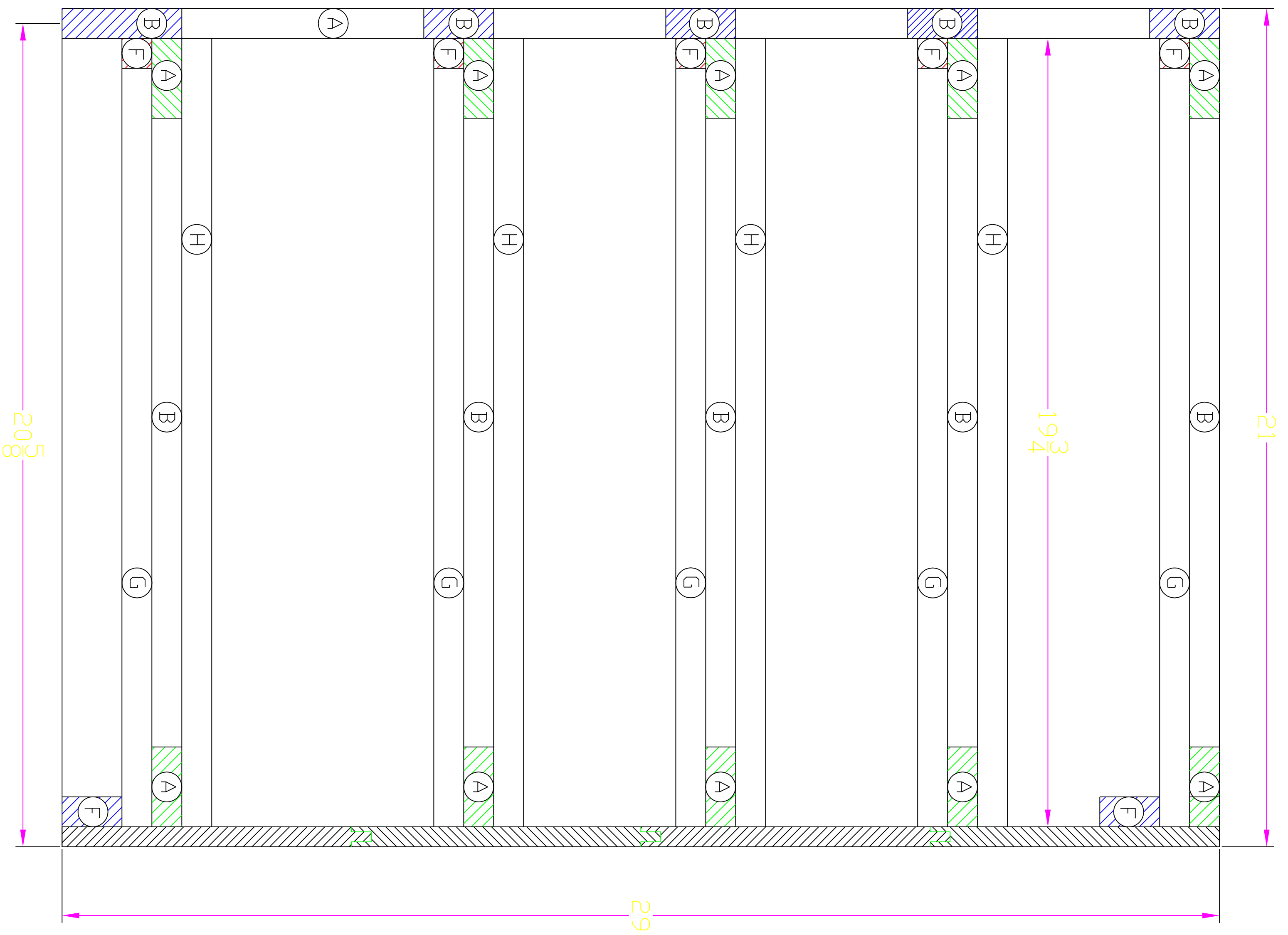
View: side view of chest showing inner drawer support frames and the frame support cleats.
