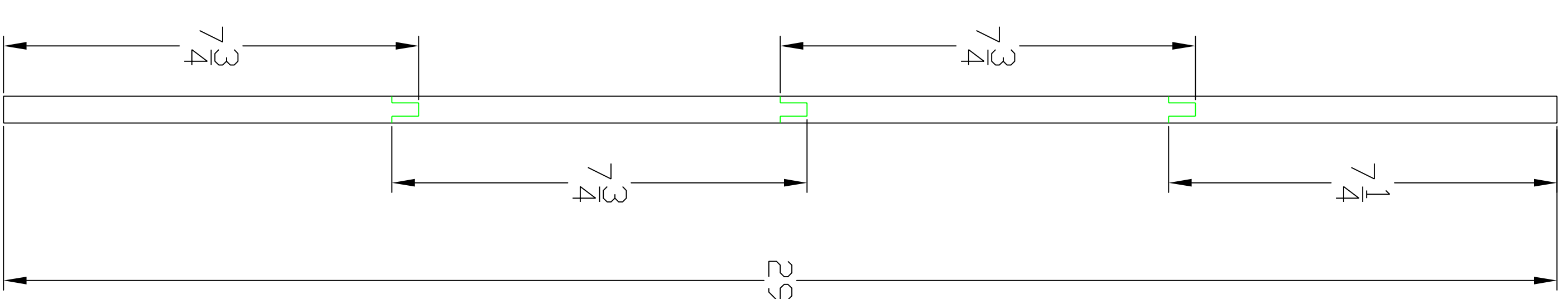
View: chest back showing tongue & groove joints and dimensions
