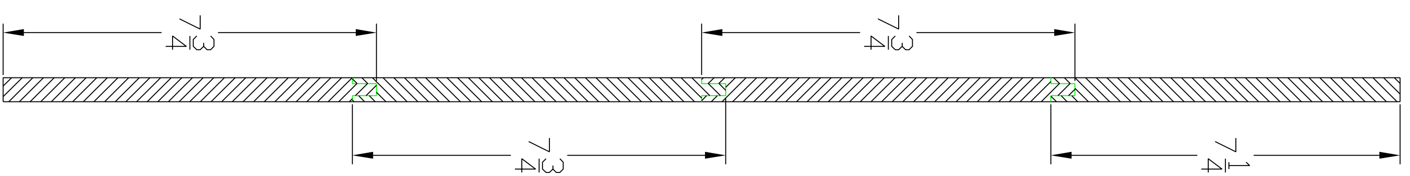
View: chest back showing tongue and groove joints
