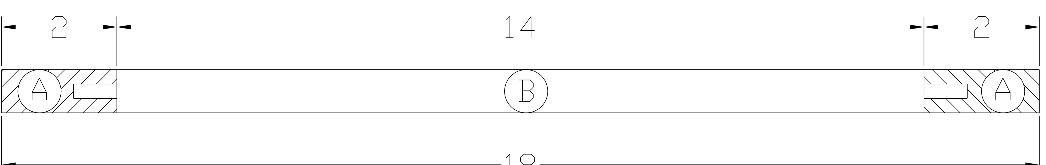
Top View of Face Frames joined with dimensions
