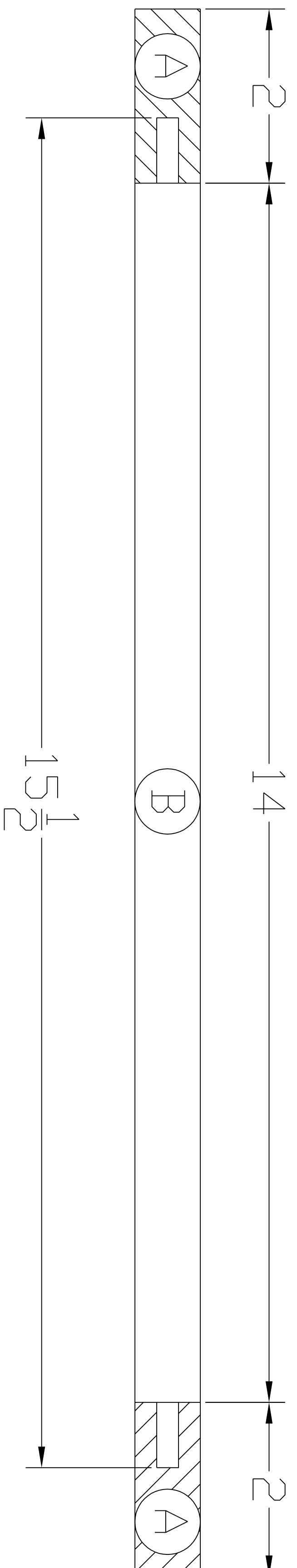
Top View of Front Face Frames joined with dimensions
