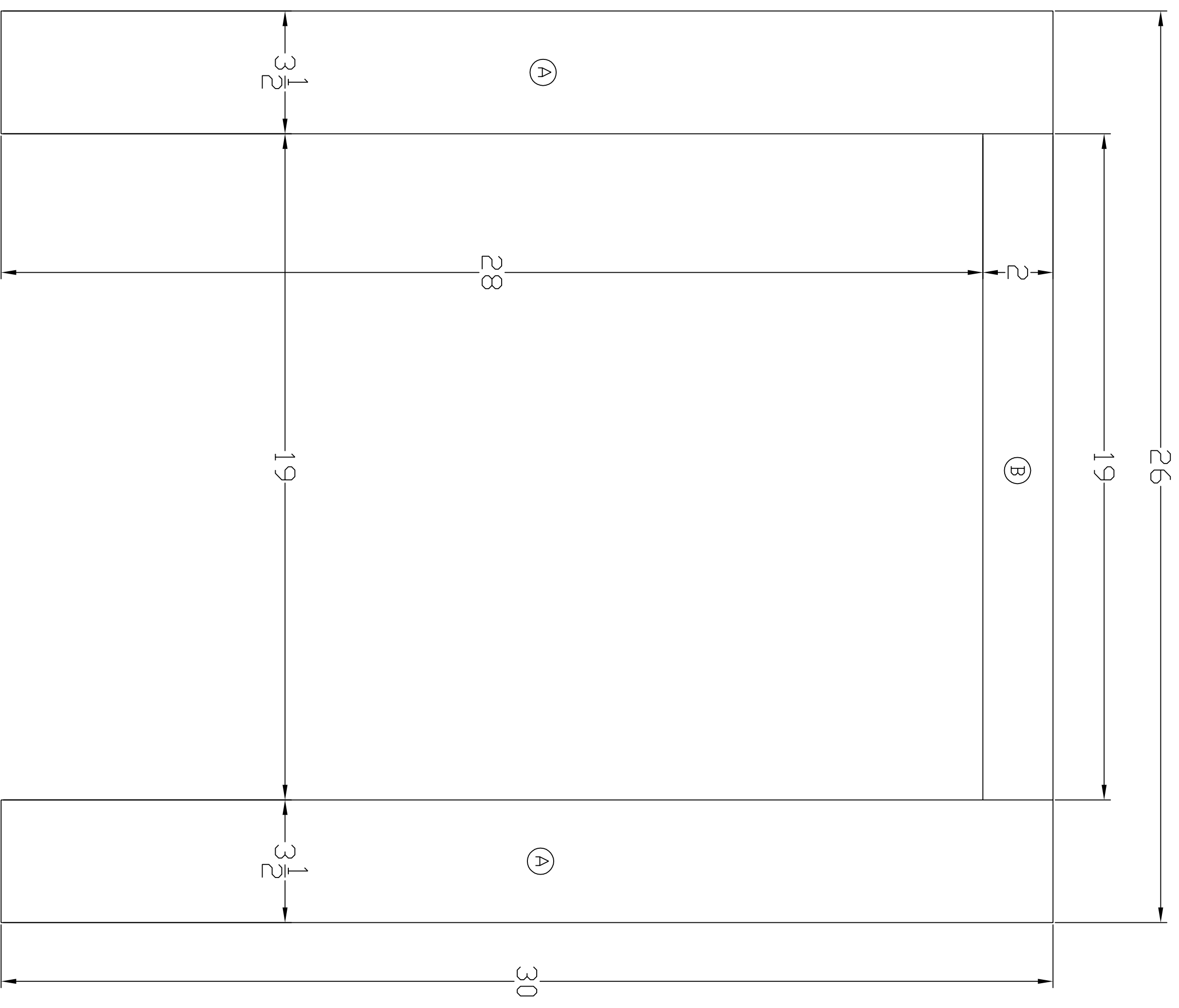
View: Maccon County Cupboard face frames with dimensions
