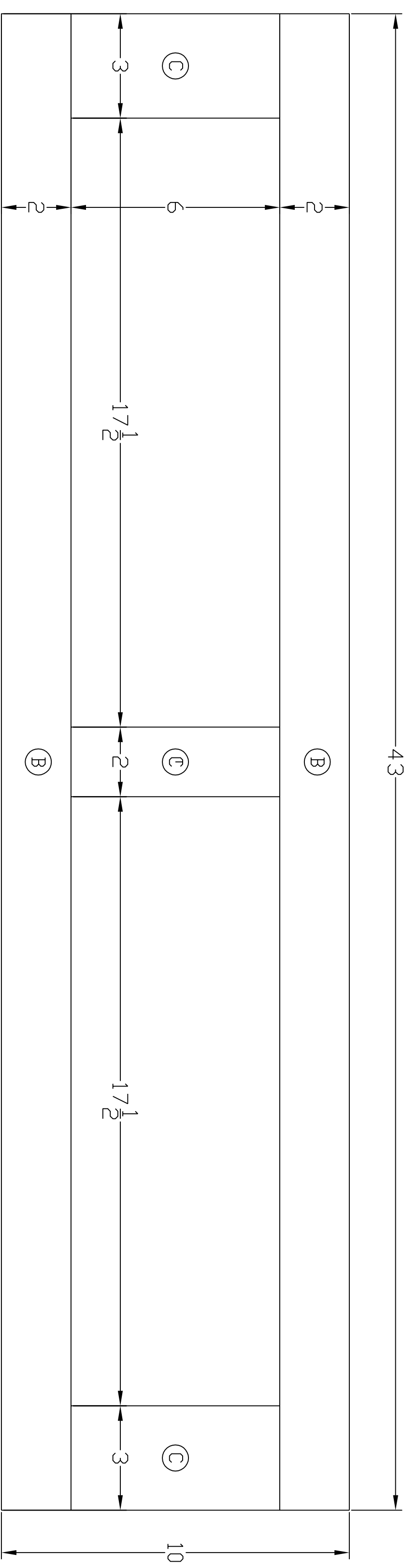
View: work station face frames closed with dimensions
